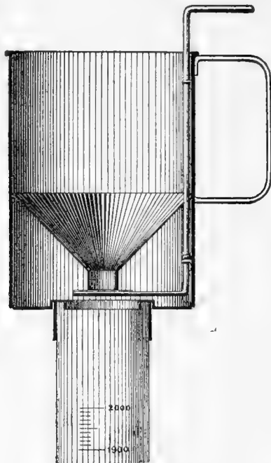
FIG. 17. Hrdlička's apparatus for measuring cranial capacity.
