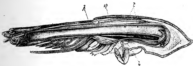
FIG. 42.—Section of Limulus rotundicauda to show the bend in the intestine with the sinewy sternal plate in the angle to be compared with that of Apus Fig. 13, p. 56. b , brain; h , heart; l , openings of the hepatic ducts in the mid-gut; sp , the sternal plate. From Bronn's Klassen und Ordnungen des Thierreiches .
