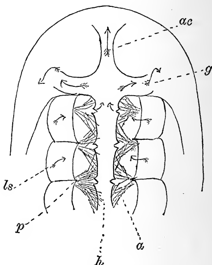
FIG. 67.—Diagram of the circulation from above. h , heart, expanded by the fine connective tissue a ; s , segmental septa forming the transverse walls of the dermo-muscular sinuses ( ls ); ac , cephalic aorta; g , lateral artery to shell and shell gland; p , points of attachment of dorso-ventral muscle bands to dorsal wall.
