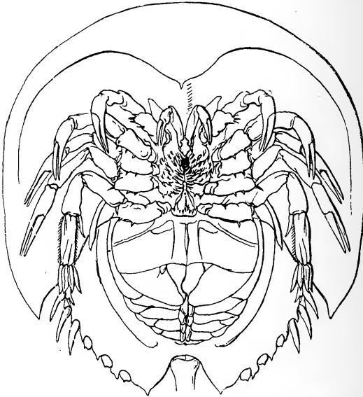
FIG. 43.—Ventral surface of Limulus moluccanus ♀ (after Van der Høeven), showing the ventral parapodia of five pairs of limbs, viz., the second, third, fourth, fifth, and sixth (first trunk limb), working between the prostomium and the under lip; also the differentiation of the sixth, or first trunk limb, for locomotory purposes.
