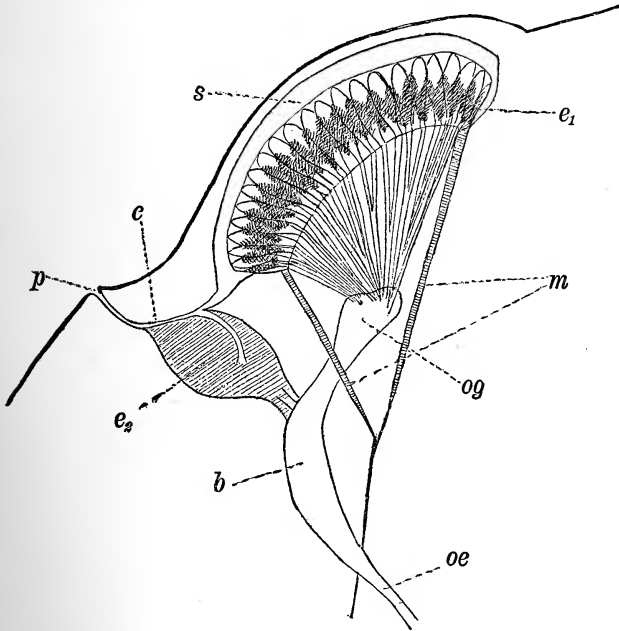
FIG. 24.—Diagram to show the water-sacs over the eyes of Apus . s , water-sacs; c , canal leading into the same; p , pore; e , paired eye; b , brain; ae , oesophageal commissure; og , optic ganglion; m , eye-muscles. The eye is drawn in the section; in reality a median section passing through the pore passes between the eyes; e 2 , unpaired eye receiving a branch from the water-canal.
