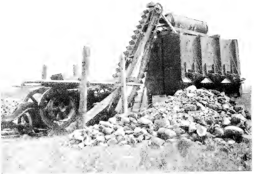
FIG. 103.—Stone-crusher in position to grind up, for road material, stones collected from the glacial drift.
