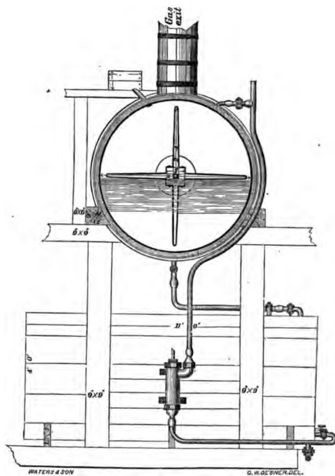
HORIZONTAL WASHER AND TANKS.—END ELEVATION AND SECTION.
