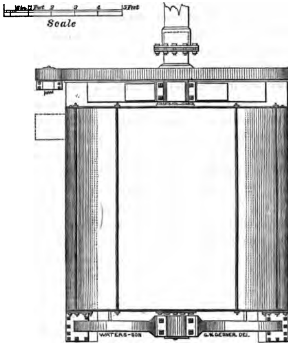
REVOLVING RETORT.—PLAN.
