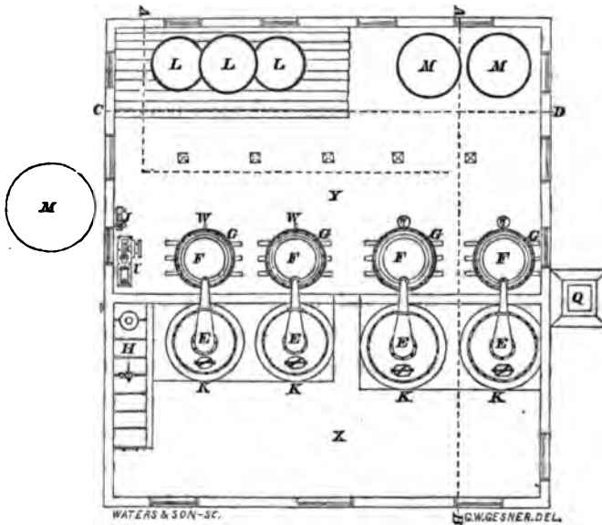
COAL OIL REFINERY PLAN.—600 GALS. CAPACITY PER DAY.
