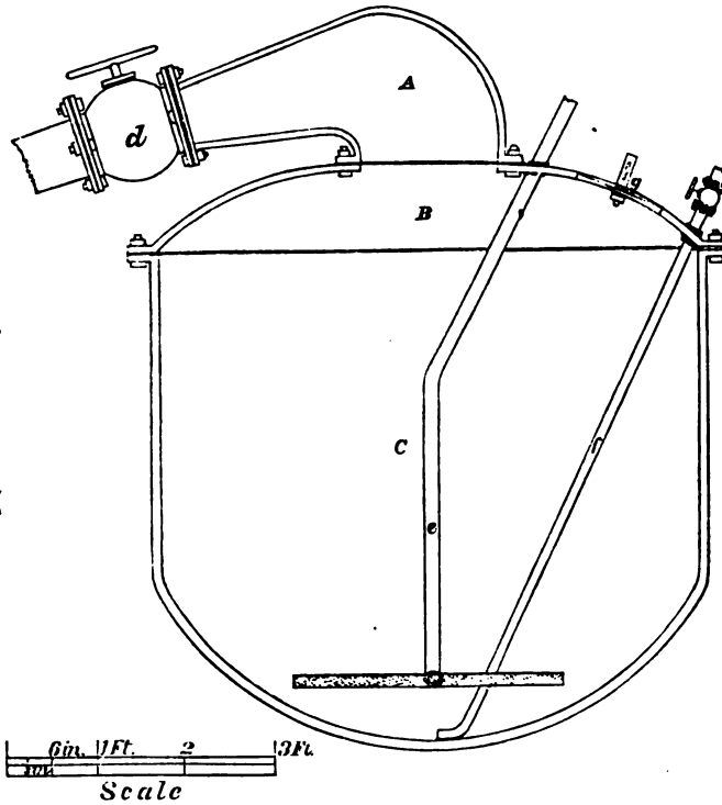
STILL.—SECTION.
