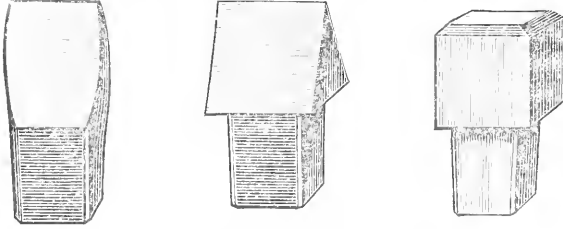
FIG. 72.—Steel Sharps and Blank, Plug shanks.
