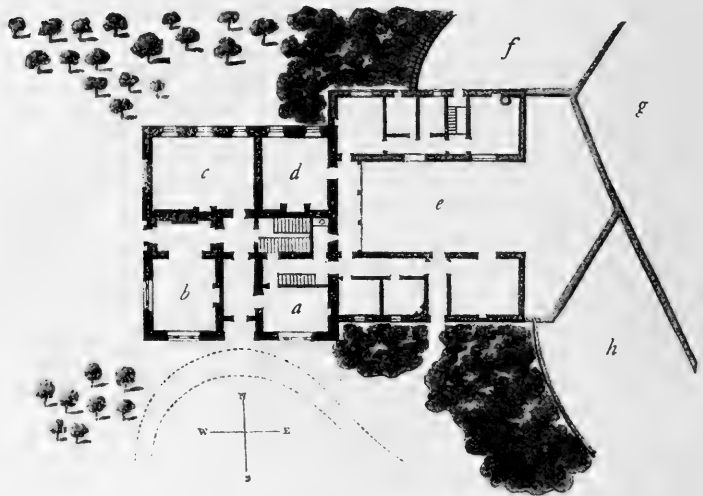
Fig. 26. Ground-plan of Villa at Brentry Hill.
