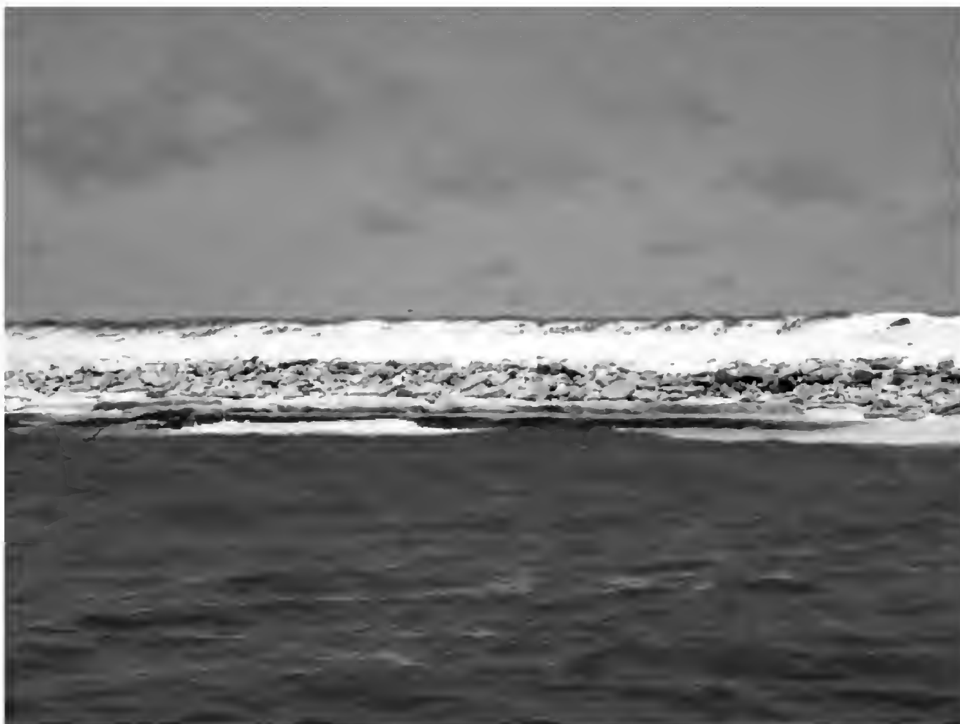
Plate 4. Steep upper beach of carbonate sands, lower boulder beach and beachrock ledges at water level on north coast, near the landing site. Note beach crest community of low herbs (photograph: Jen Ashworth, January 2005).
