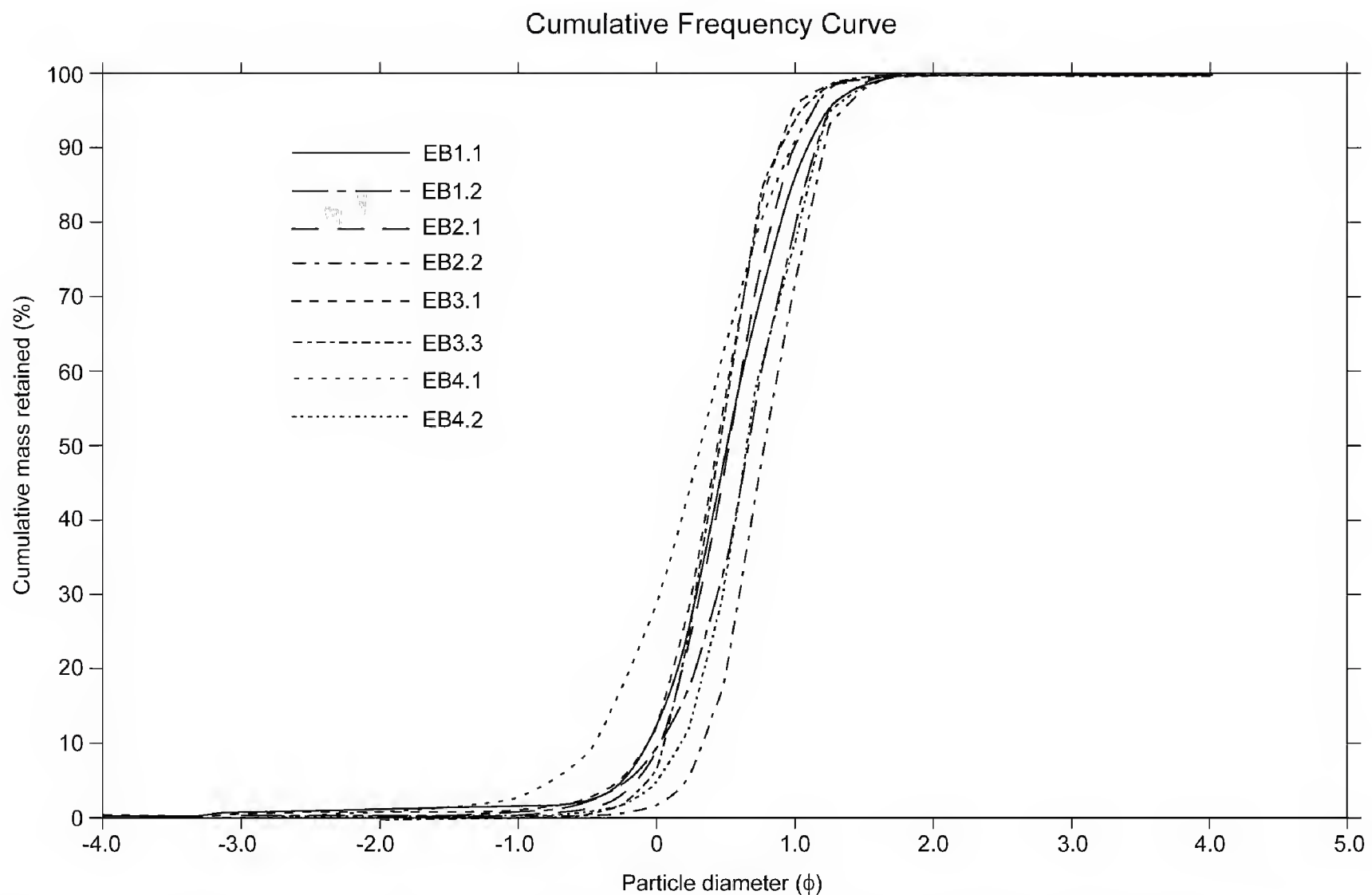
Figure 2. Cumulative frequency curves for sediment samples from upper and lower beaches.
