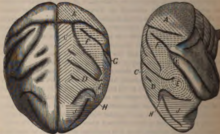
FIG. 236 (After Munk). Upper Surface of the Brain of the Monkey. —Sensory Areas: A, of the eyes; B, of the ears; C, of the sensibility of the lower extremity; D, Anterior extremity; E, Head; F, Ocular muscular apparatus; G, Region of ears; H, Neck; I, Body.
