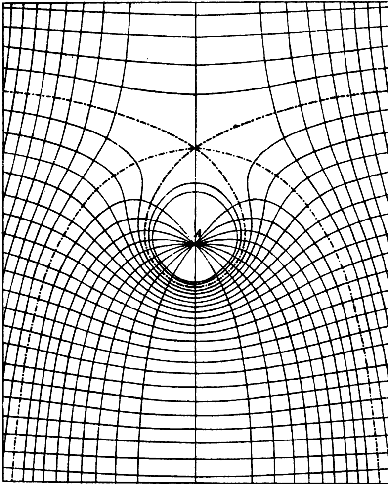
Lines of Force and Equipotential Surfaces.
