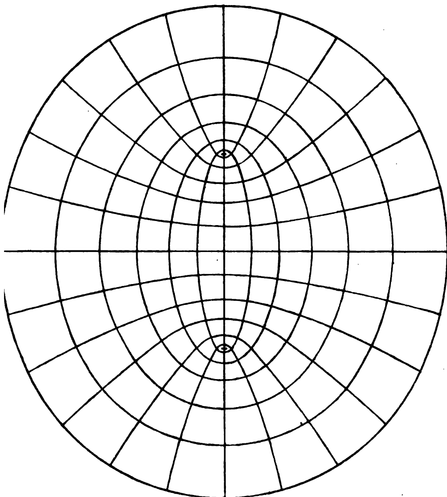
Confocal Ellipses and Hyperbolas
