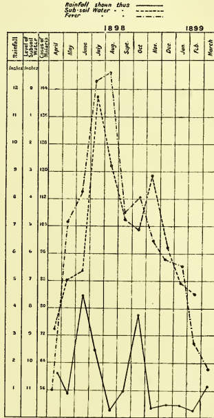
RAINFALL, SUB-SOIL WATER AND FEVER AT LAGOS
