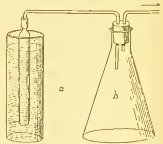
FIG. 31.—Chamberland's candle and flask arranged for filtration.
