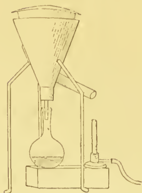
FIG. 7.—Hot-water funnel.
