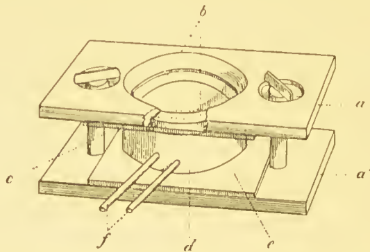
FIG. 28.—Graham Brown's chamber for anaerobic hanging-drops (A portion of one edge of upper plate is shown cut away.)
