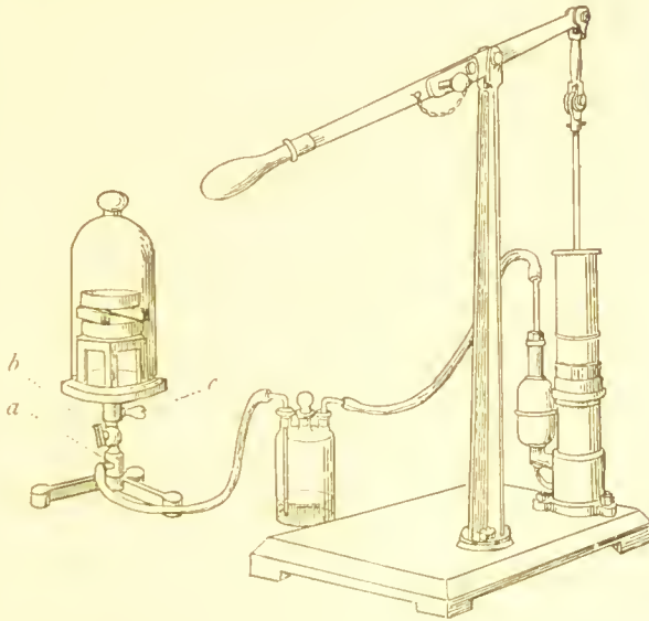
FIG. 37.—Geryk's air-pump for drying in vacuo .
