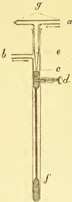
FIG. 38.—Reichert's gas regulator.
