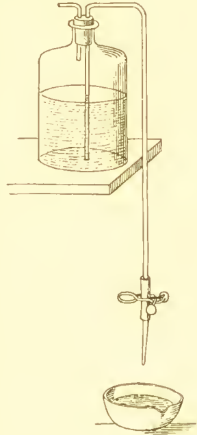
FIG. 42.—Syphon wash-bottle for distilled water used in washing preparations.
