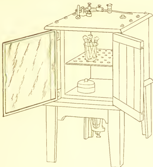
FIG. 39.—Hearson's incubator for use at 37° C.
