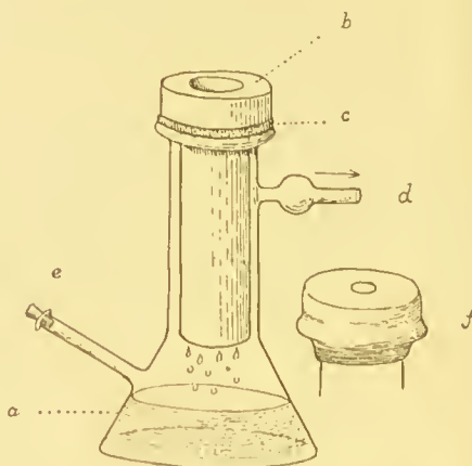
FIG. 34.—Mucenke's modification of Chamberland's filter.
