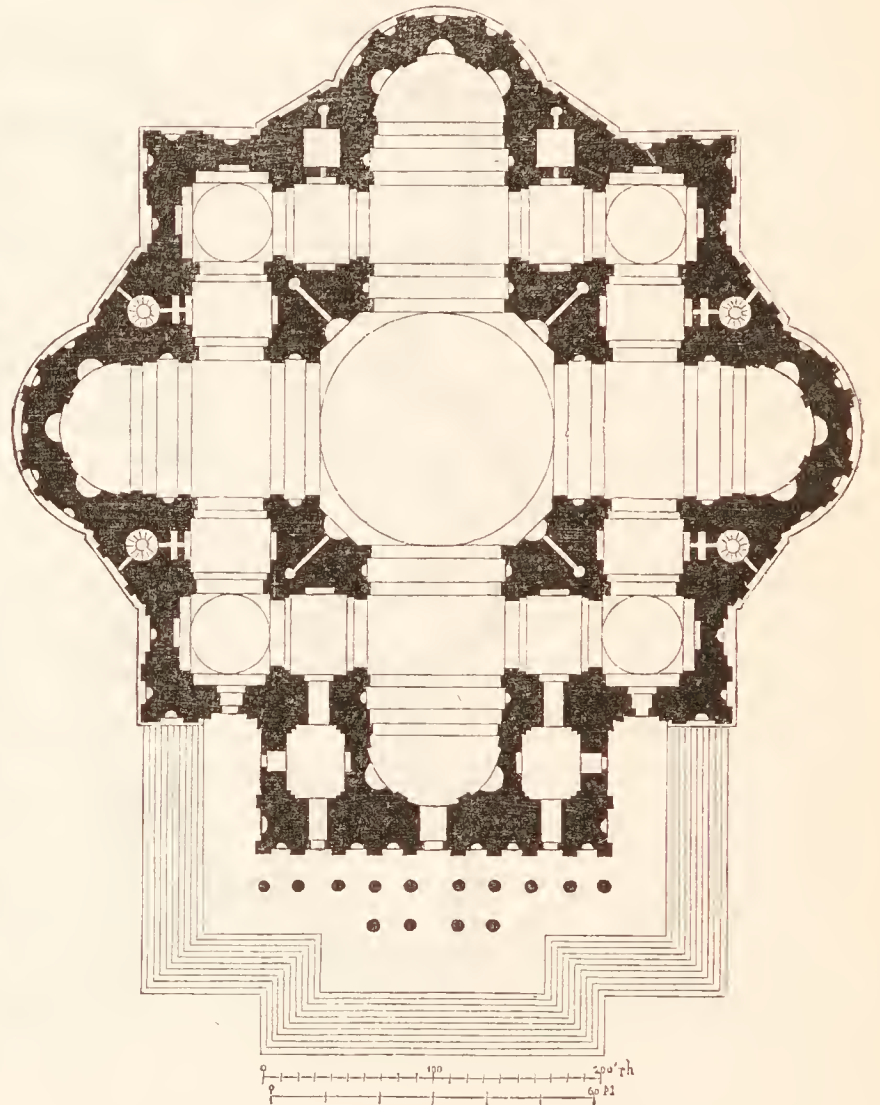
Fig. 86. St. Peter. Michelangelo's Grundriss.
