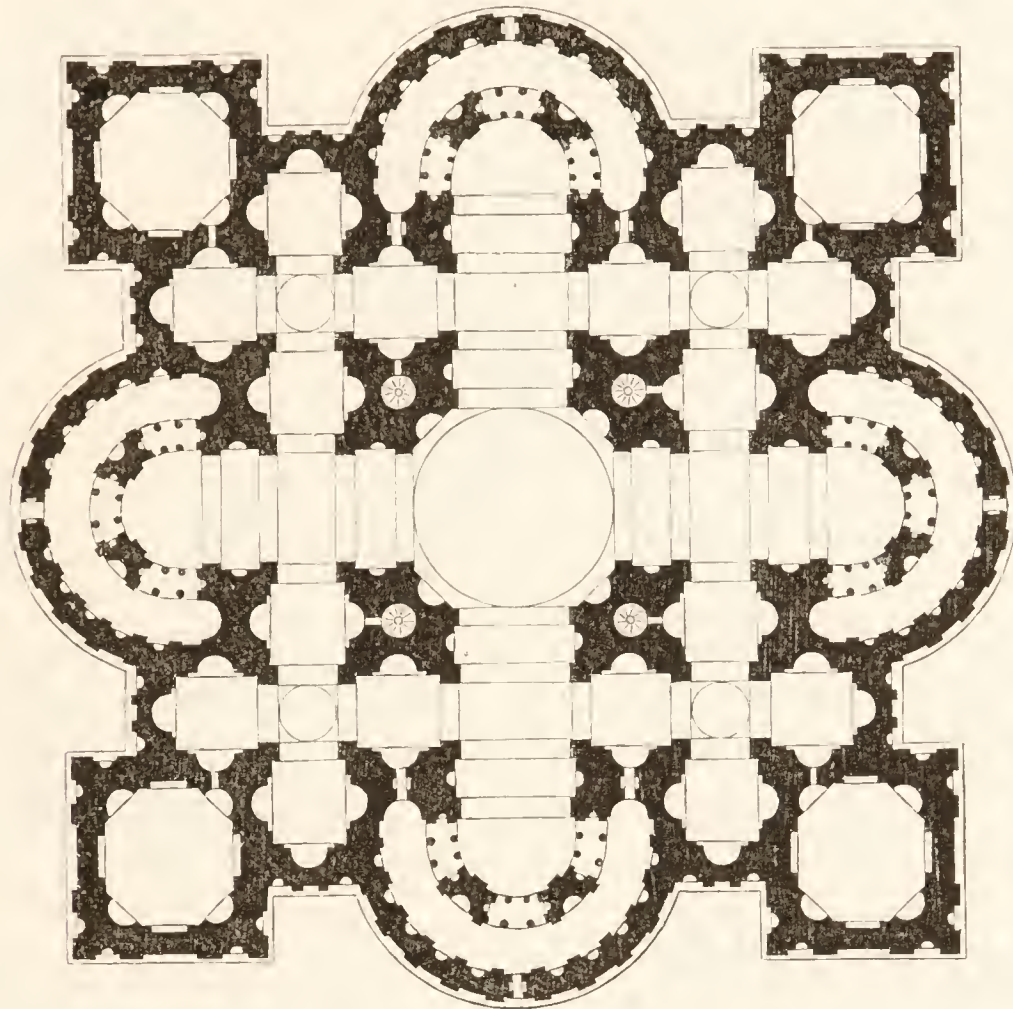
Fig. 84. St. Peter. Peruzzi's Grundriss.
