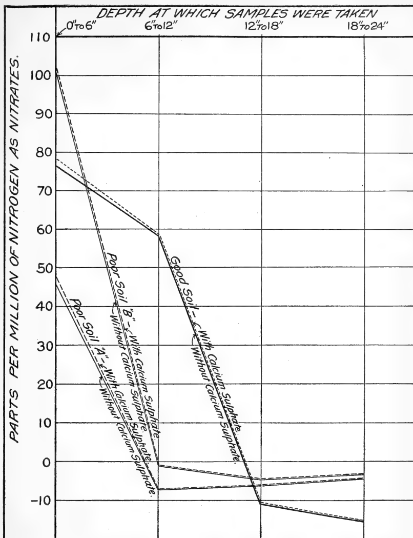
FIG. 18.—Diagram showing the effect of calcium sulphate upon nitrication of ammonium sulphate in samples of soil from plat 300, Truckee-Carson Experiment Farm, representing poor soil "A"; plat 310, representing poor soil "B"; and plat 320, representing good soil.
