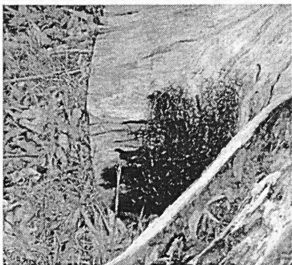
The black patch is a swarm of crane flies
