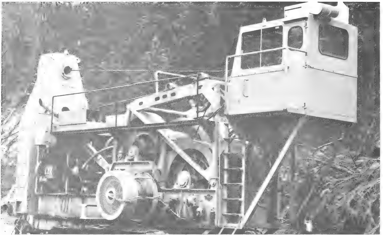
Figure 10.--Washington Model 608A yarder.
