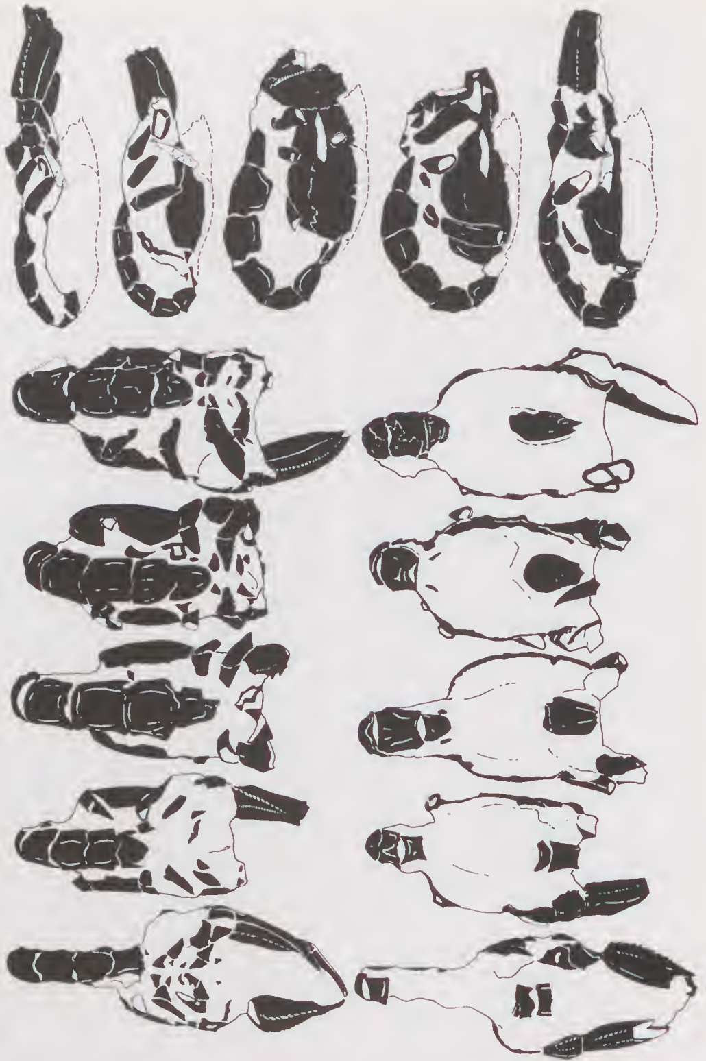
Fig. 5. A range of Thalassina fossils showing little variation in the relative positions of body parts. The similarity of all fossil mudlobsters configurations demonstrates the moulting process is the likely cause.
