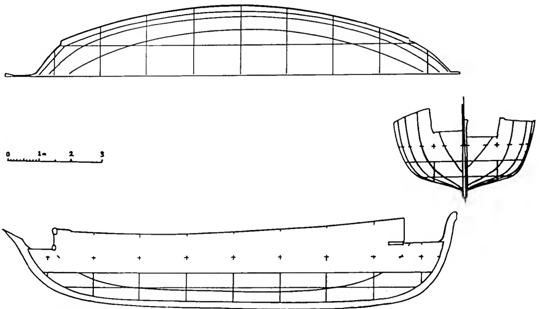
Fig. 2. Proposed lines for a perahu padewakang .
