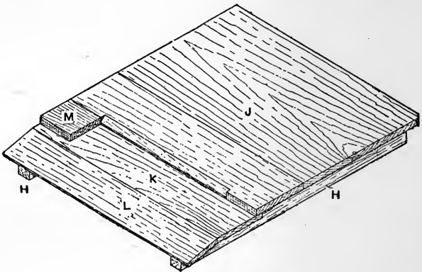
Fig. 22.—Floor-board.
