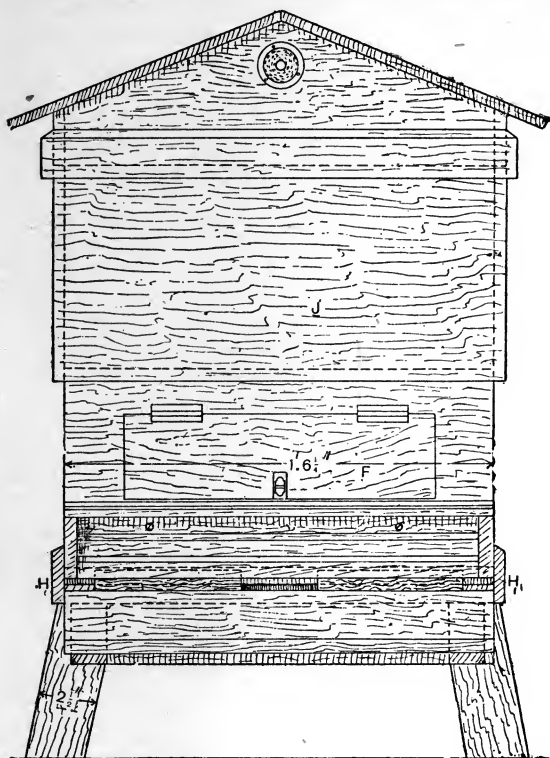
Fig. 68.—Front Elevation of Observatory Beehive.
