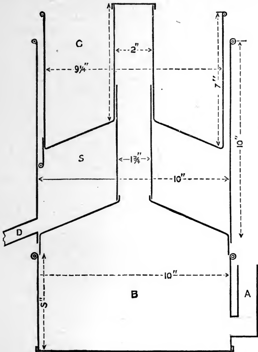
Fig. 130.—Section of Gerster Wax Extractor.
