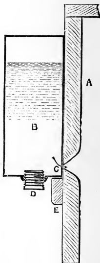
Fig. 139.—Section of Hone Dummy Feeder.
