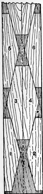
Fig. 23.—Cutting Beehive Roof Gables.
