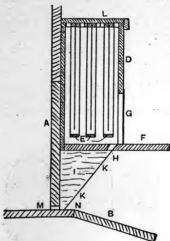
Fig. 145.—Section of Swarm Catcher.
