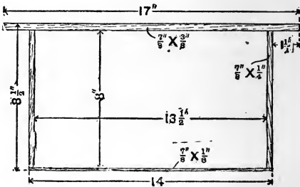
Fig. 34.—B.B.K.A. Standard Frame.
