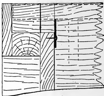
Fig. 28.—Section of Top Edge of Front and Back of Body-box.
