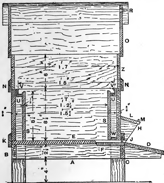
Fig. 2.—Longitudinal Section of Bar-frame Beehive.
