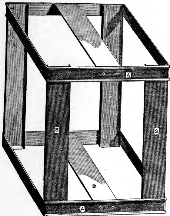
Fig. 121.—Bands, Slides and Bridges of Extractor.
