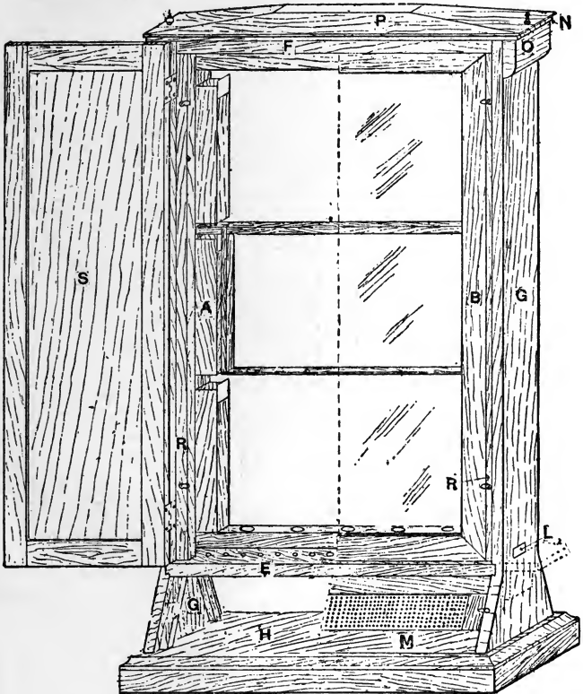
Fig. 69.—Observatory Beehive for Temporary Use.
