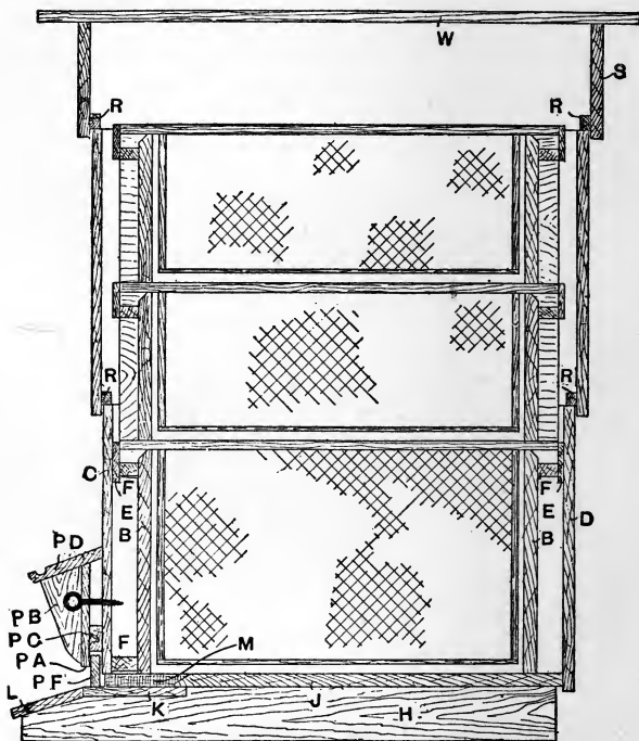
Fig. 16.—Longitudinal Section of Tiering Bar-frame Beehive.
