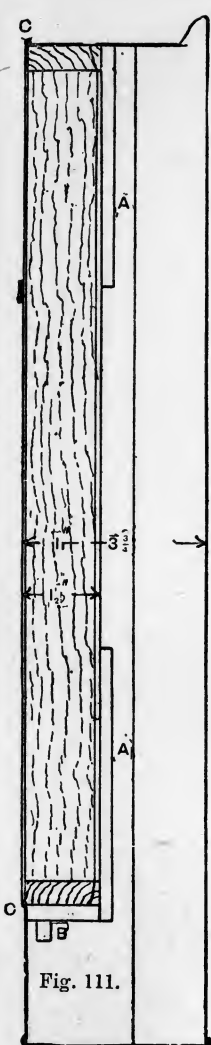
Figs. 111 and 112.—Section and Front View of Little Wonder Can and Cage.
