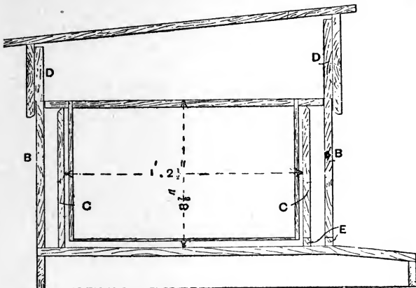
Fig. 84.—Plan of Body-box.
