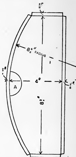
Fig. 113.—Pattern for Top and Bottom of Extractor.
