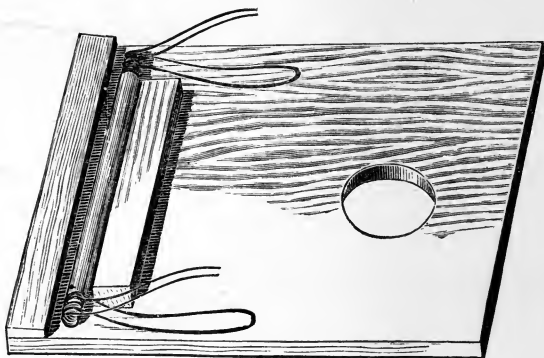
Fig. 102.—Bottom Board of Bellows.
