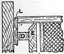
Fig. 13.—Device to Prevent End-shake to the Frames.
