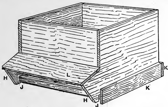
Fig. 4.—Brood Chamber Outer Casing.
