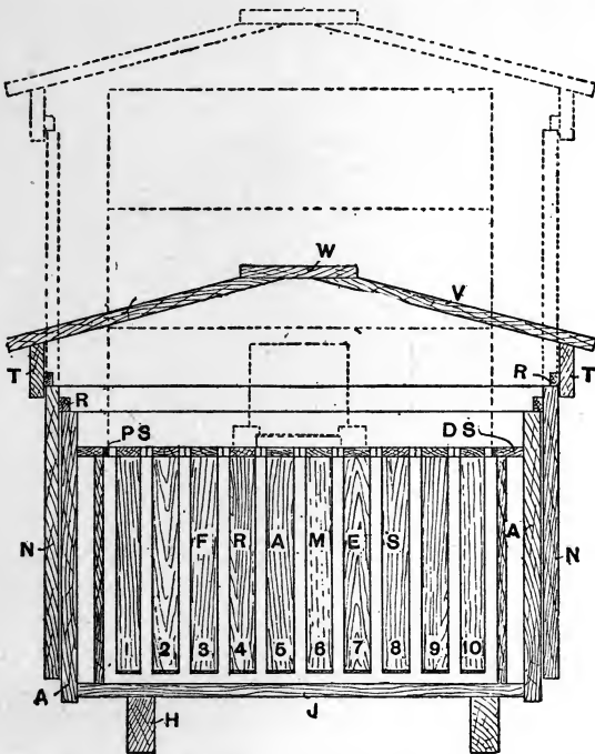
Fig. 17.—Cross Section of Tiering Bar-frame Beehive.
