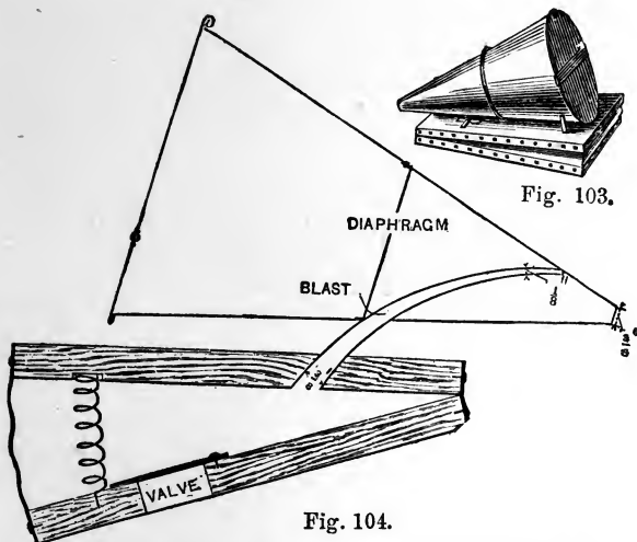
Fig. 103.—Clarke Smoker. Fig. 104.—Section of Clarke Smoker.
