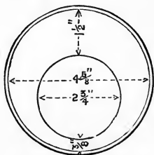
Fig. 106.—Bottom of Funnel.
