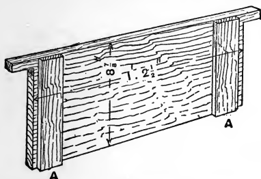
Fig. 58.—Simple Form of Dummy.
