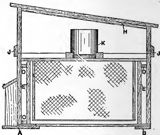
Fig. 10.—Section of Temporary Beehive.
