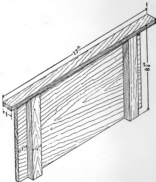
Fig. 56.—Back View of Dummy.
