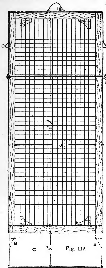
Figs. 111 and 112.—Section and Front View of Little Wonder Can and Cage.
