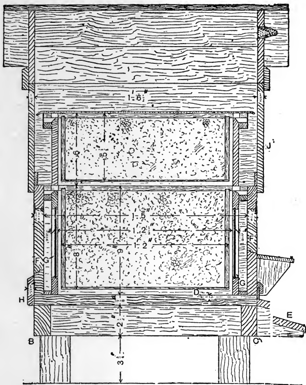
Fig. 66.—Vertical Section through Observatory Beehive.
