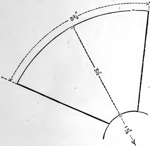
Fig. 96.—Pattern of Funnel.
