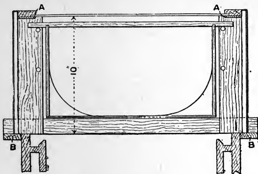
Fig. 77.—Section of Inspection Case.
