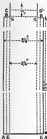
Fig. 120.—Pattern of Slide.
