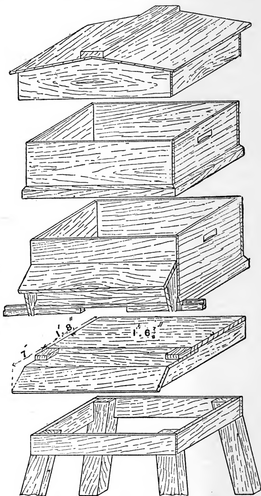
Fig. 25.—Parts of "W.B.C." Beehive.
