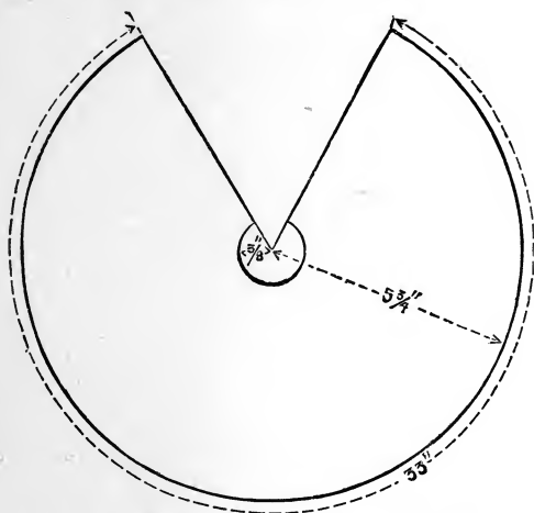
Fig. 131.—Pattern for Cylindrical Top of Boiler.
