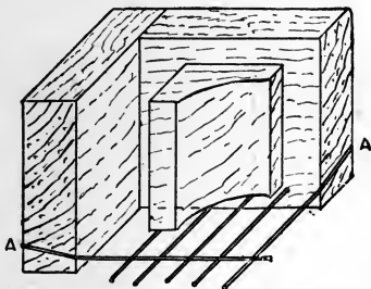
Fig. 114.—Corner of Cage of Little Wonder Extractor
