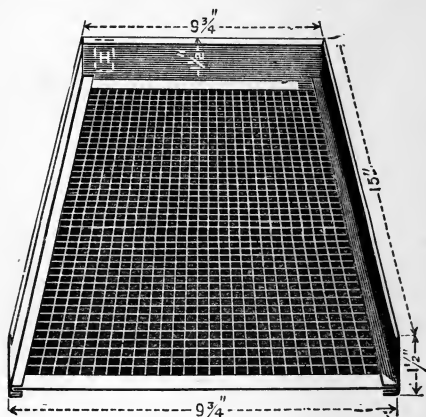
Fig. 122.—Half of Comb Basket.
