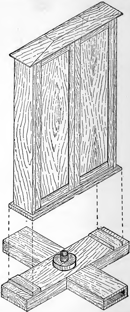
Fig. 75. —Mounting Observatory Beehive on Feet with Pivot.
