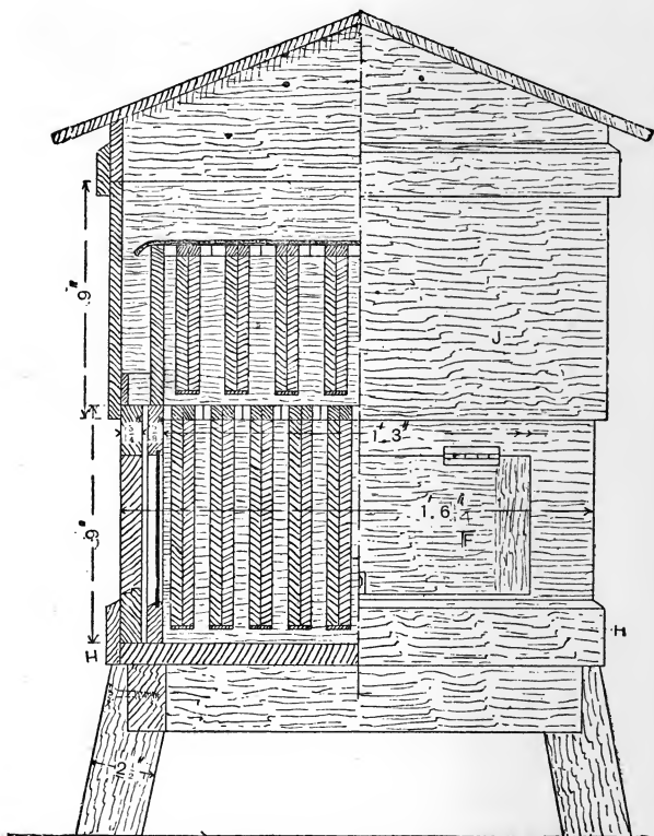
Fig. 67.—Half Cross Section and Half Back Elevation of Observatory Beehive.
