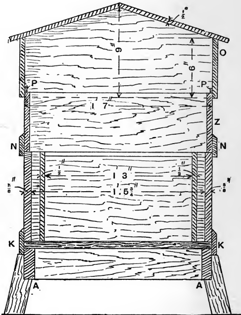
Fig. 1.—Cross Section of Bar-frame Beehive.
