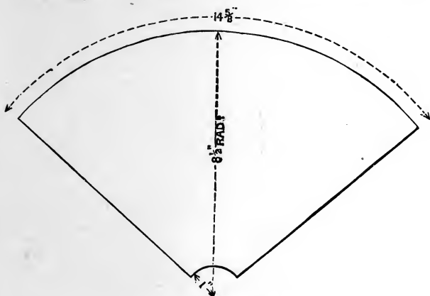
Fig. 105.—Pattern of Funnel.
