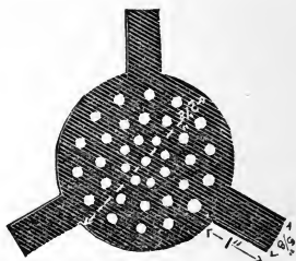
Fig. 97.—Smoker Diaphragm.
