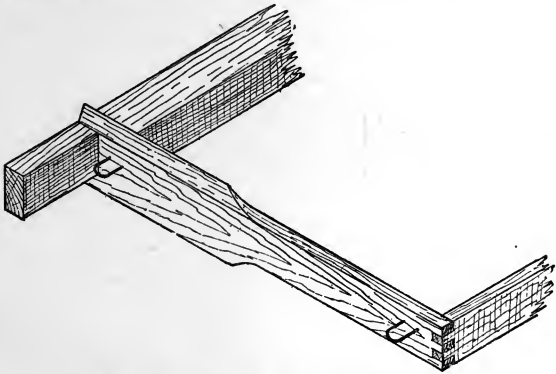
Fig. 55.—Staples used as End Spacers.
