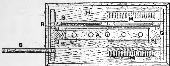
Fig. 71.—Horizontal Section of Observatory Beehive.
