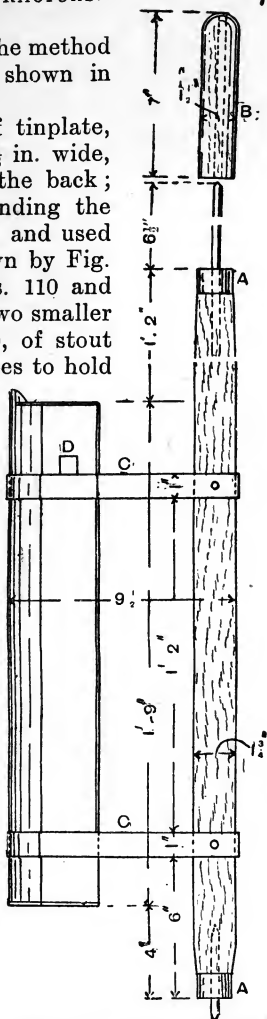
Fig. 108.—Little Wonder Honey Extractor.
