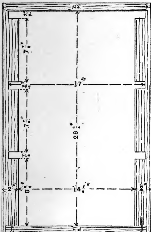
Fig. 73.—Inside Frame of Observatory Beehive.
