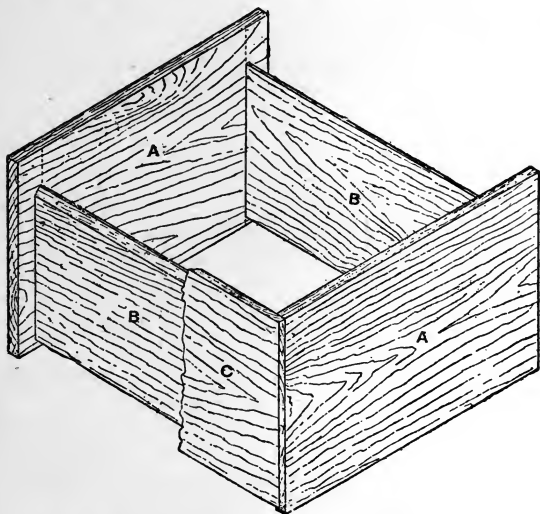
Fig. 19.—Body-box of Tiering Bar-frame Beehive.
