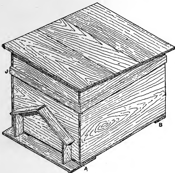
Fig. 9.—Temporary Beehive.
