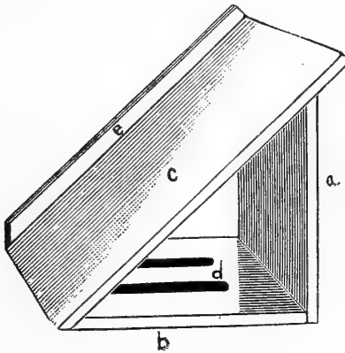
Bevel-Gauge.
