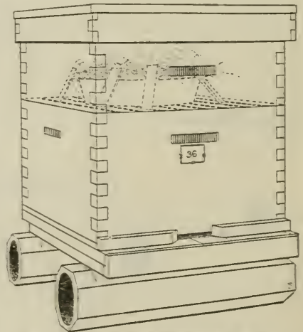
FIG. 20.—Pan in super arranged for feeding.
