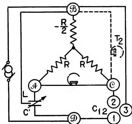
Fig. 4—Null-Impedance Bridge Method for Direct Capacity
