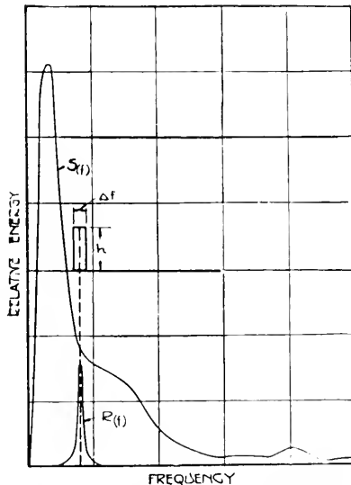
Fig. 3—Illustrating Correction of Observations, Necessary Because of Variation in Resolving Power with Frequency Setting
