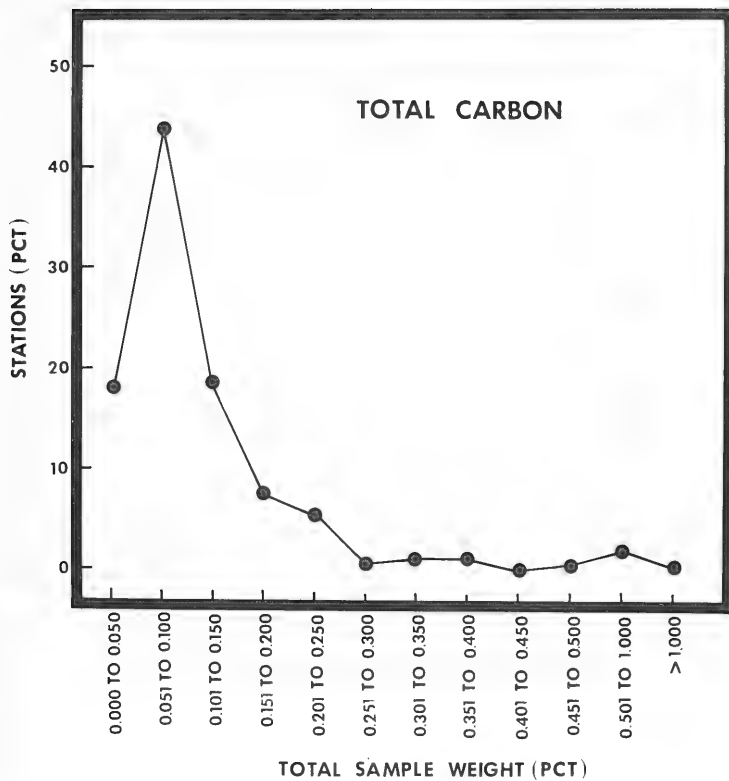
Figure 13. Percentage frequency of total carbon at all stations.
