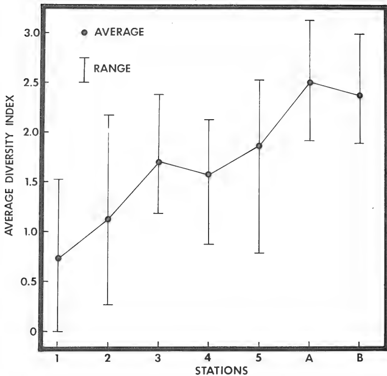
Figure 31. Average and range of diversity indexes at the five transect stations and stations A and B.
