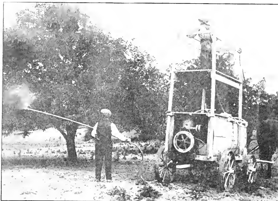
Power sprayer arranged to reach both the upper and lower parts of the tree.
