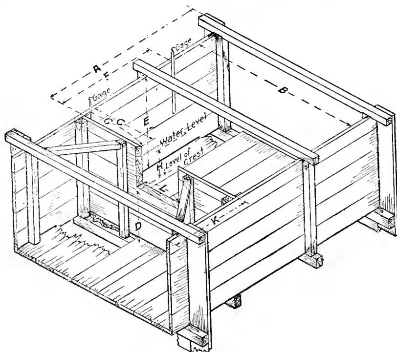
Fig. 1. Plan of weir box.
