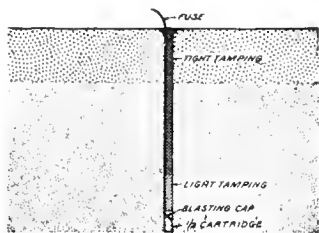
Fig. 5. Top of hole tamped tight.
