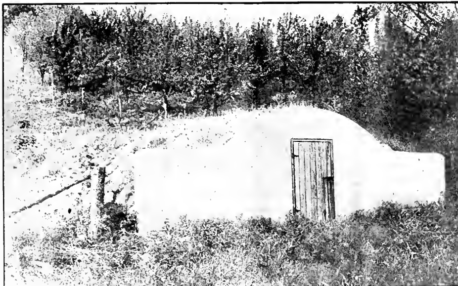
Fruit and vegetable storage cellar (exterior view). This illustration gives view of a storage cellar at Purdue University, Lafayette, Indiana. Its dimensions are 50 feet long by 10 feet 6 inches wide. It is built of concrete and the method of construction is the Van Guilder hollow-wall type. It has three ventilators of six-inch tile and cost $400 when completed.
