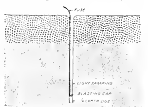
Fig. 4. Light tamping over charge.
