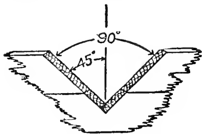
Fig. 4. Triangular notch weir.
