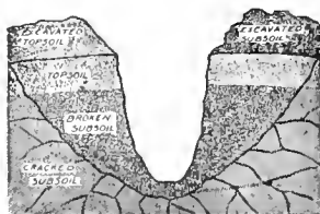
Fig. 7. The best practice is to shovel out the loose soil and expose the pothole. This is easily done in the freshly blasted holes.
