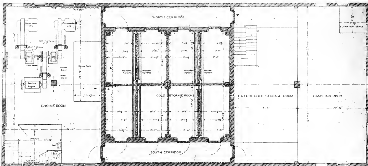
FIGURE 2—First floor plan of experimental cold storage plant, showing engine room, refrigeration chambers, unfinished refrigeration space and handling room.
