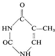
Thymine (5-methyl-2:6-dihydropyrimidine)
