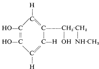
Adrenaline (epinephrine)
