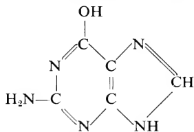
Guanine (2-amino-6-hydroxypurine)
