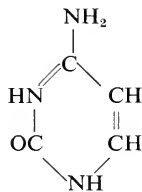
Cytosine (2-hydroxy-6-aminopyrimidine)
