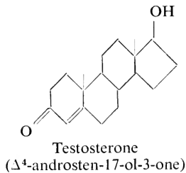
The tetracyclic carbon skeleton in androgens
