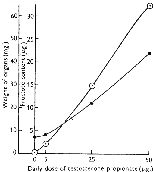
FIG. 13. Dosage-response curves of testosterone propionate, using the coagulating glands of the rat; \circ — \circ , fructose ( \mu\text{g.} ); \bullet — \bullet , weight of organs (mg.).
