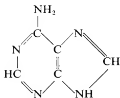
Adenine (6-aminopurine)
