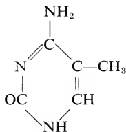
5-Methyl-cytosine
