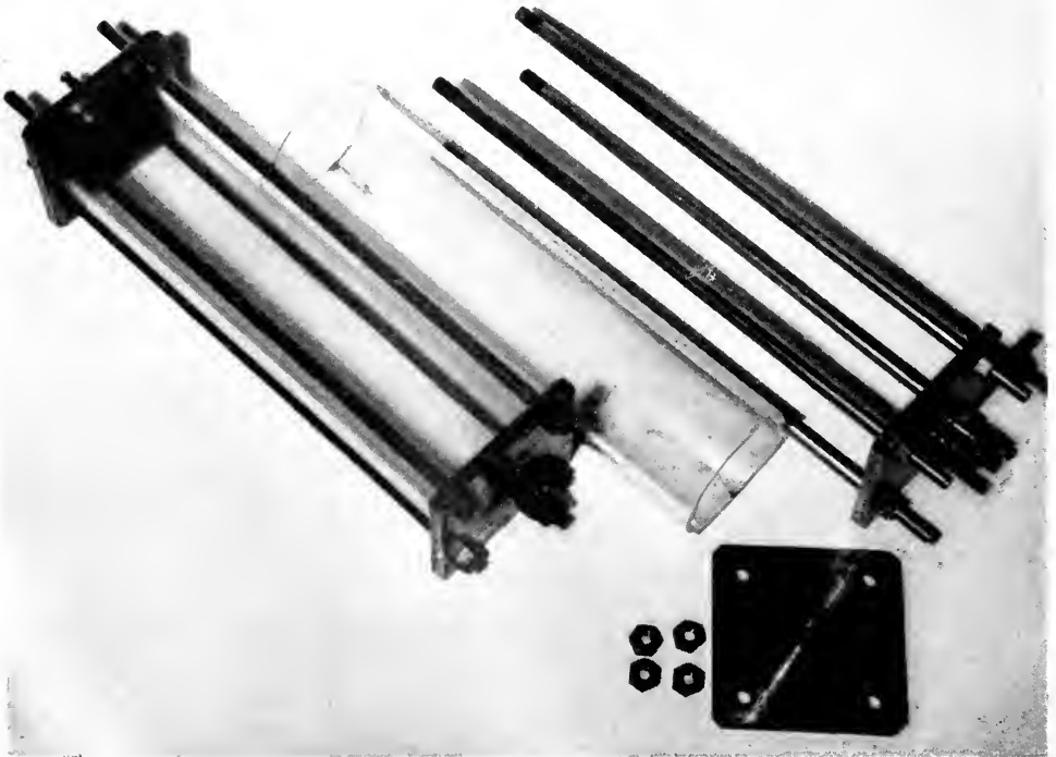
FIGURE 2. A 3460-cc. Lucite compensation chamber and its component parts.
