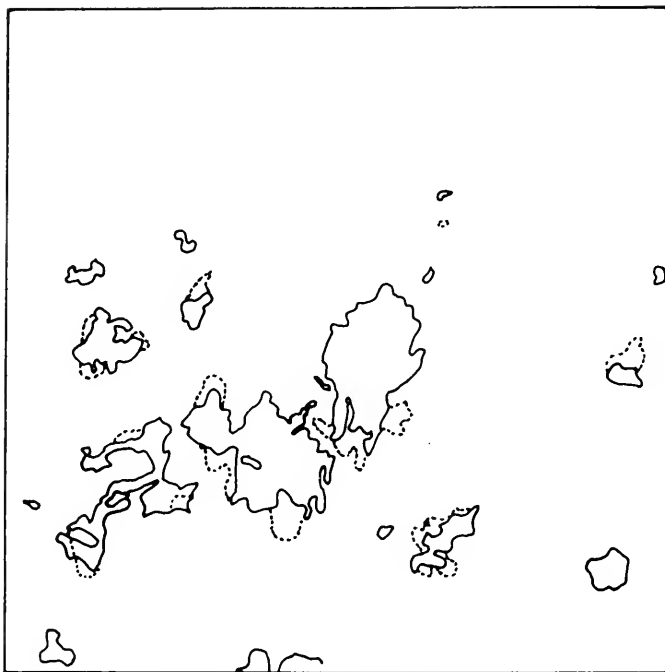
FIGURE 1. Changes in outlines of patches of Eurypon sp. taken from color photographs over the period June, 1975 (—) to February, 1982 (---) in a 25 cm 2 area of the Sponge Garden.
