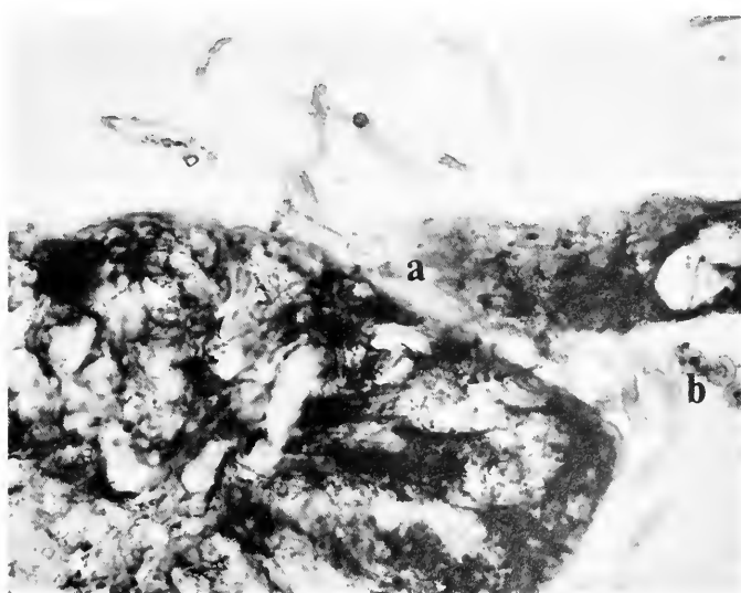
FIGURE 5. Closer view of infecting hyphae: a) hypha proliferation in the coral epithelium, and b) misplaced zooxanthellae PAS. 400 \times .
