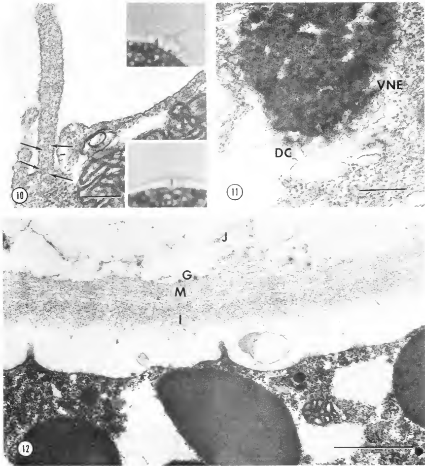
FIGURE 10. Higher magnification electron micrograph showing microfilaments (arrows) longitudinally-arranged in the microvilli of the fertilization cone. Bar = 0.25 \mu m. Insets: light micrographs showing late stages in fertilization cone formation. In the upper inset, the sperm tail still protrudes from the fertilization cone; in the lower inset, the sperm tail has been lost.
