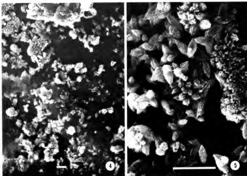
FIGURE 4. Scanning electron micrograph of the shell window, 48 hours of regeneration, showing small crystals associated with an organic matrix. Bar = 10 \mu m.
