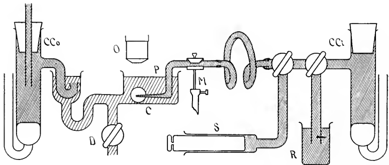
FIG. 1. Diagram of apparatus. The egg, impaled on the capillary pipette P , lay in a chamber C beneath the microscope objective O . Outside electrical contact was made through a calomel half cell CC0 which dipped into the solution in which the egg was immersed at some distance from the egg, and drainage of the chamber was effected through the tube D at an intermediate point. The movements of the pipette were controlled by a Chambers micromanipulator M . The pipette is in communication through a coil of hard rubber tubing not only with the other calomel half cell CC1 , but also with a Luer syringe S for pressure control, and with a reservoir R , the height of which was adjustable.
