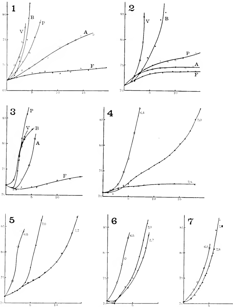
FIGS. 1-7: Swelling curves for Arbacia eggs in half molar solutions of various ammonium salts. Abscissae, times in minutes; ordinates, diameters in arbitrary units each equal to 1.064\mu . (See Footnote I concerning the pH values used.)
