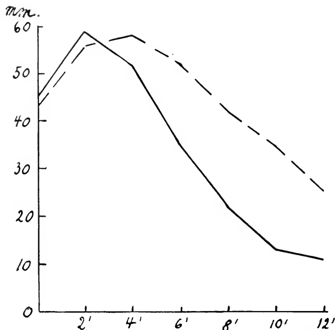
FIG. 1. The course of fatigue in a pair of sartorii stimulated in 0.111\text{ M NaCl} + 10.2\text{ M} \times 10^{-3}\text{ KCl} + 8.1\text{ M} \times 10^{-4}\text{ CaCl}_2 (—) and in 0.103\text{ M NaCl} + 10.2\text{ M} \times 10^{-3}\text{ KCl} + 64.4\text{ M} \times 10^{-4}\text{ CaCl}_2 (---).
