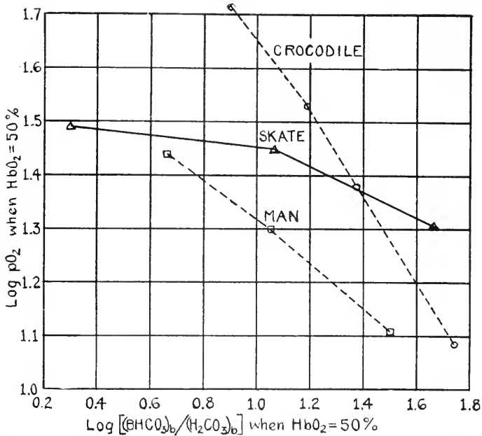
FIG. 3. Position of the oxygen dissociation curves (log p\text{O}_2 when \text{HbO}_2 = 50 per cent) in relation to log (\text{BHCO}_3)/(\text{H}_2\text{CO}_3) .
