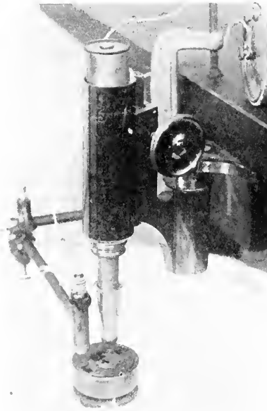
FIG. 3. Near view of rotor on stator with microscope and illumination.
