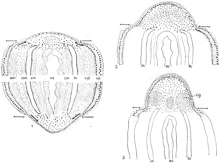
FIGS. 1-3, Lincus socialis .
