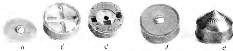
FIG. 1. Rotors for air turbine. (a) cover for tube type; (b) tube type rotor showing grooves for centrifuge tubes; (c) rotor for microscope observation; (d) tube type rotor with cover on; (e) bottom of rotor showing flutings.
