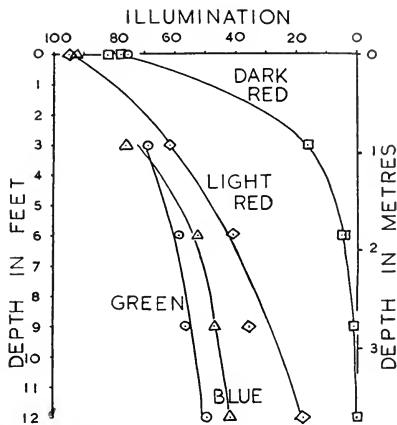
FIG. 3. Graph showing illumination at various depths in open water at position A , on the west side of Carsaig Island (see inset to Fig. 1). Color filters were used in addition to opal glass. The illumination in air is rated as 100. The observations were made on August 19, 1936.
