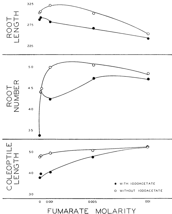
FIG. 5. Relationship between coleoptile length, root number and root length and the concentration of fumarate with and without .00001 M iodoacetate.
