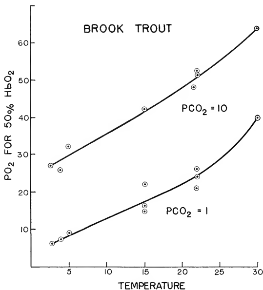
FIG. 4. The effect of temperature upon the pressure of oxygen necessary to half-saturate blood of brook trout at CO 2 tensions 1 and 10 mm.
