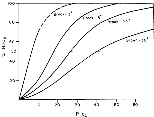
FIG. 2. Oxygen dissociation curves of trout blood at various temperatures.
