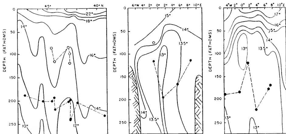
FIGURE 15. Noon scattering layer depths and temperature profiles. (Azores temperatures modified from Iselin, 1936; Western Mediterranean temperatures from Bumpus, 1948.) a. Azores area (July-Aug.). b. Western Mediterranean (Jan.). c. Western Mediterranean (Apr.-May).
