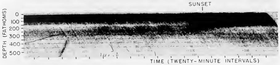
FIGURE 17. Bathygram showing evening ascent of one scattering layer and the simultaneous descent of another. Atlantis cruise 149, 7 July, 1947; noon position: 38^{\circ}42'N. , 69^{\circ}32'W.
