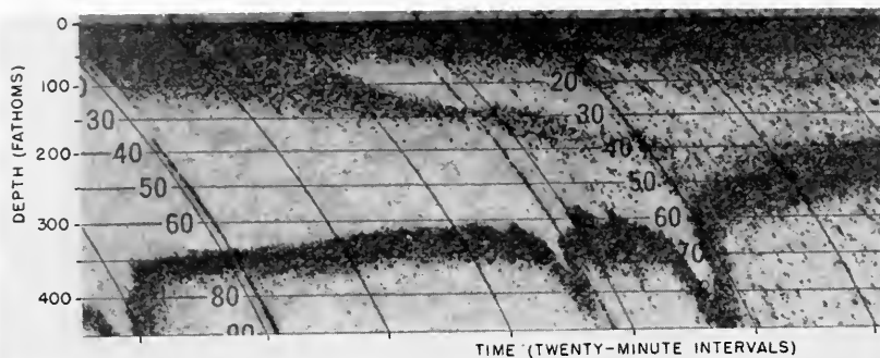
FIGURE 9. Bathygram showing morning descent of scattering layer onto bottom at 200 to 250 fathoms. Atlantis cruise 154, 7 Apr., 1949; 25^{\circ}51'N , 79^{\circ}41\frac{1}{2}'W .
