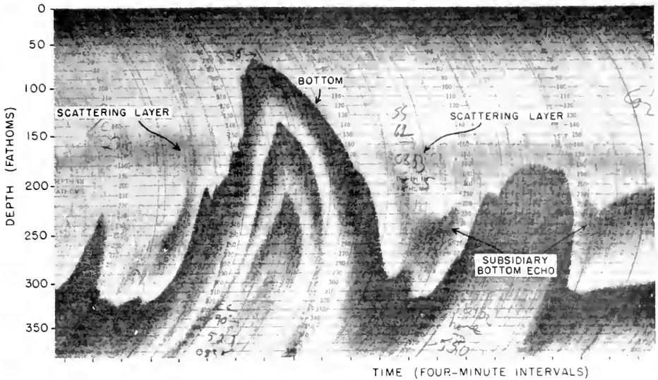
FIGURE 7. Bathygram showing scattering layer (160 to 190 fathoms) interrupted by submarine peak. Atlantis cruise 156, 4 June, 1949; 38^{\circ}11'N. , 73^{\circ}30.5'W.
