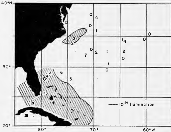
FIGURE 27. Observed distribution of E. americana and proposed boundary of illumination only.
