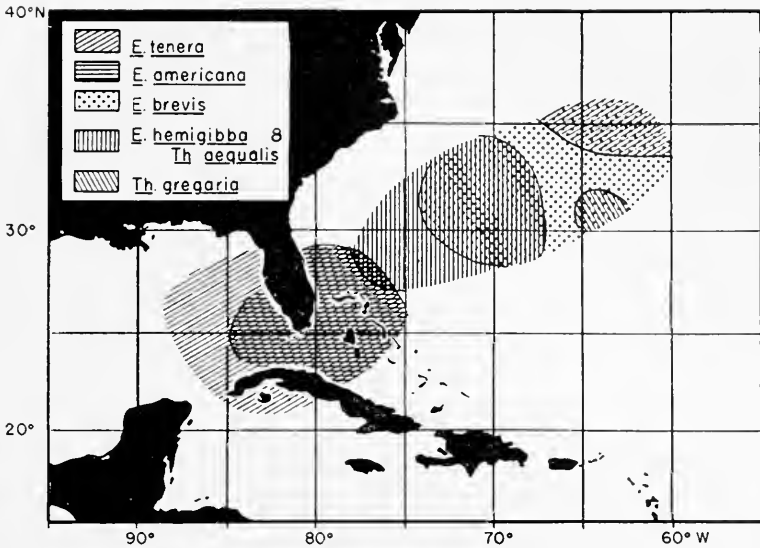
FIGURE 3. Areas of dominance of euphausiid species in Western Atlantic. (Information is lacking in unshaded areas.)
