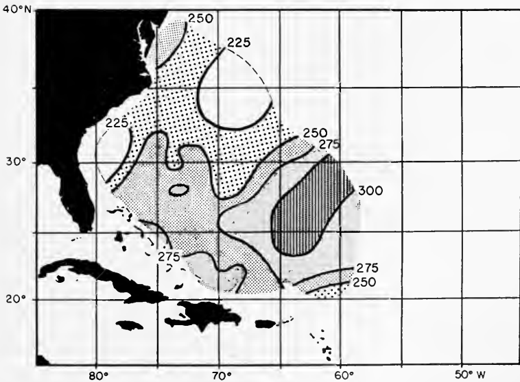
FIGURE 4. Geographical trend of the noon depth of the scattering layer. (Figures represent the corrected approximate depth in fathoms of the peak abundance of scatterers.)
