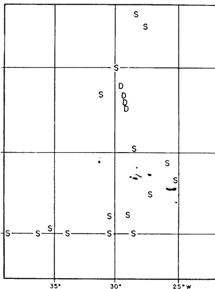
FIGURE 6. Occurrences of double and single echo in the Azores area.
