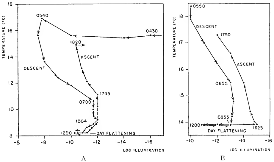
FIGURE 23. Conditions of temperature and illumination experienced by a scattering layer in the course of its diurnal migration. (Figures show local apparent time.) a. Atlantis cruise 144, 24 Feb., 1947; 25°26'N., 93°44'W. b. Atlantis cruise 144, 13 Jan., 1947; 21°21'N., 75°39'W.
