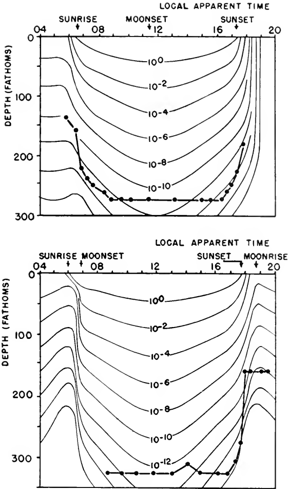
FIGURE 14. Diurnal migration of scattering layer showing marked noon flattening. a. Atlantis cruise 144, 13 Jan., 1947; noon position: 21°21'N., 75°39'W. b. Atlantis cruise 143, 11 Oct., 1946; noon position: 26°04'N., 60°55'W.
