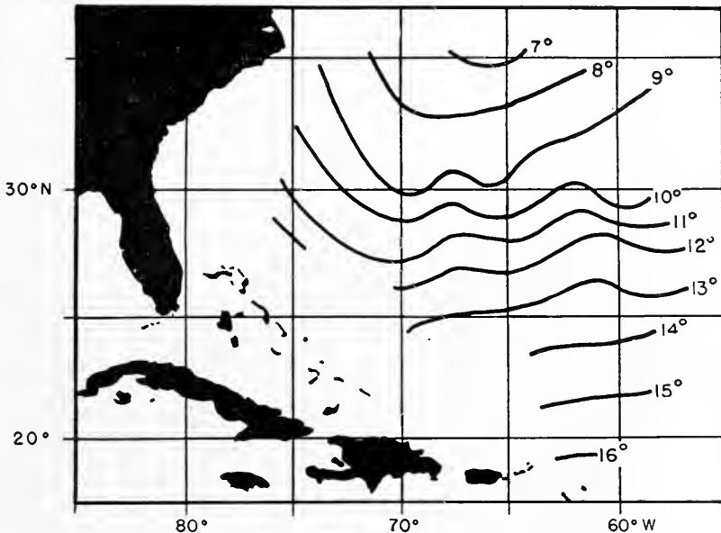
FIGURE 20. Difference in temperature ( ^{\circ}\text{C} ) in summer between the surface and a depth of 328 fathoms.
