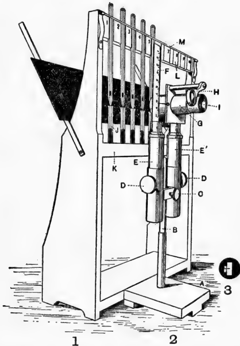
FIG. 104.—Apparatus for quantitative estimation of specific precipitation. (Nuttall and Inchley, in "Journal of Hygiene.")
