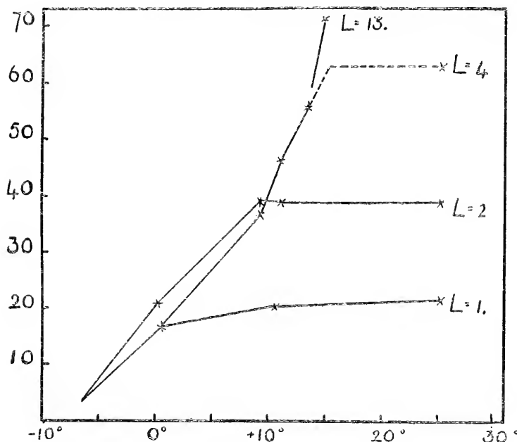
FIG. 13.—Light, temperature and assimilation; each graph represents the course of assimilation (mgs. \text{CO}_2 per 50 sq. cm. per hour) with rising temperature for a given light intensity ( L = 1, 2, 4, 13 ): in each, assimilation rate rises till light becomes limiting, and then the graph takes a horizontal course: the exact point of inflection for L = 4 is conjectural, and this part of the graph is dotted: light = 13 is not limiting for the highest temperature ( 15^\circ \text{C} ) for which a value is given. (After Matthaei, modified.)
