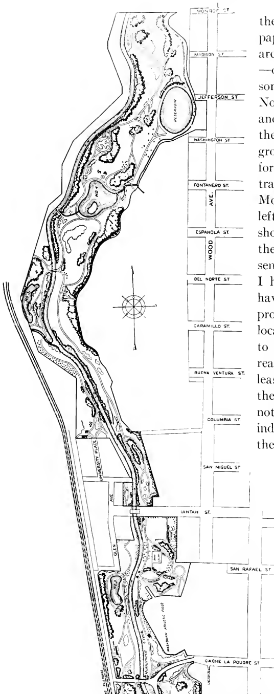
MAP OF THE NORTHERN PORTION OF MONUMENT VALLEY PARK, COLORADO SPRINGS, COLO. Copied from the map in the Report of the Park Commission for 1908. The city blocks are 400 feet square, streets 100 feet wide.
