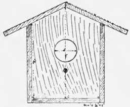
PROFESSOR BAILEY'S SUGGESTIONS FOR BIRD-HOUSES. (After Cornell University Experiment Station.)
