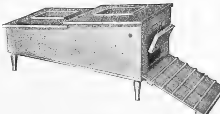
"Buckeye" 25-Chick Lampless Brooders No. 5. INDOOR.
