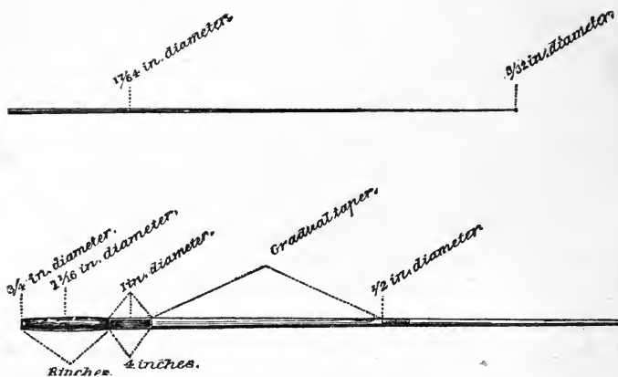
The Henshall Black Bass Rod.—(Specifications.) (Abbey & Imbrie.)
