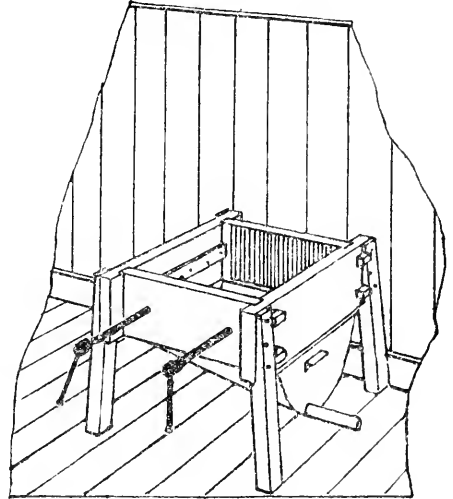
Fig. 1.—Elevation.
