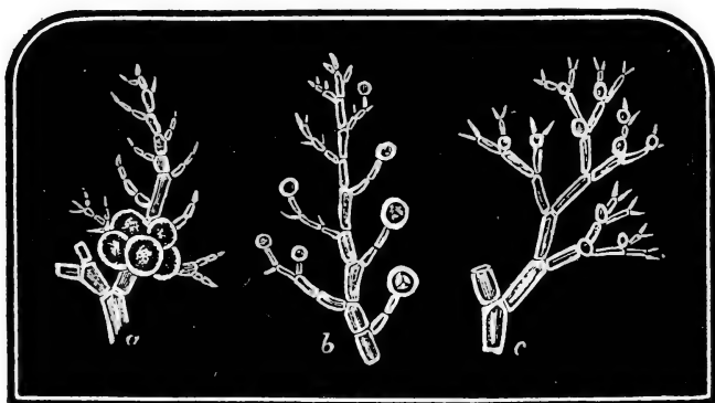
FIG. 202. (a) Magnified branchlets of C. gracillimum , with favellæ; (b) the same, with tetraspores; (c) C. granulatum .
