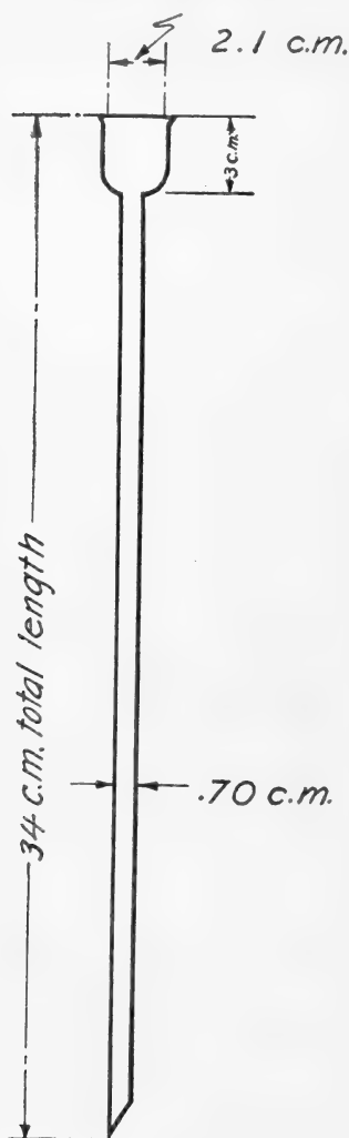
FIG. 13.—Condenser tube
