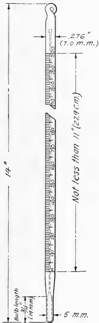
FIG. 4.—Standard thermometer with the proper shape and dimensions for use in the Brown-Duvel moisture tester
