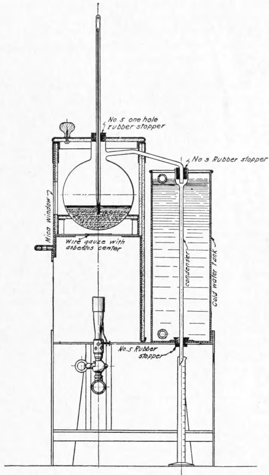
Sectional view of the official moisture tester, showing the various parts properly connected for use.
