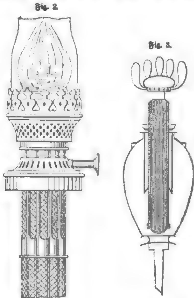
Mitraillusenbrenner.
