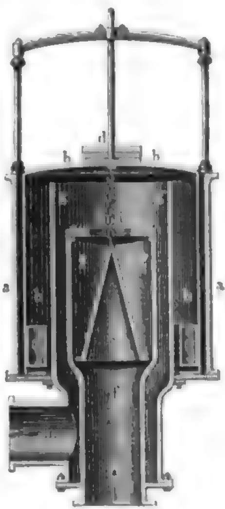
Fig. 8. Regulator.
