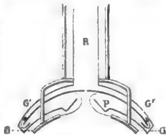
Siemens' Automatabrenner.
