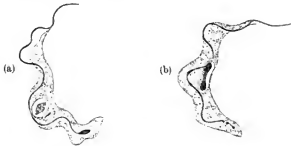
Fig. 2. Trypanosoma equinum .
