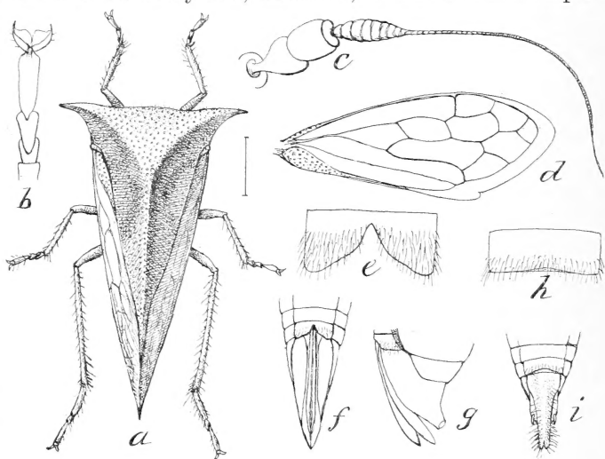
FIG. 1.—BUFFALO TREE-HOPPER: female ( a ), with enlargement of foot ( b ), antenna ( c ), wing ( d ), ovipositor ( f , g ), and terminal segment of male abdomen ( h , i ) (author's illustration).
