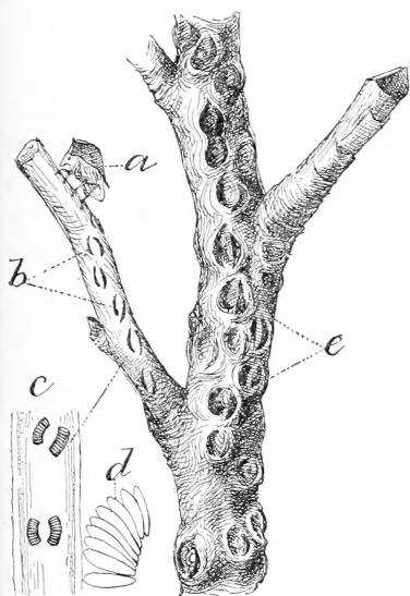
FIG. 4.— Ceresa bubalus .: twig of apple showing: a, female at work; b, recent egg-punctures; c, bark reversed with eggs in position, slightly enlarged; d, single row of eggs still more enlarged; e, wounds of two or three years' standing on older limbs (author's illustration).
