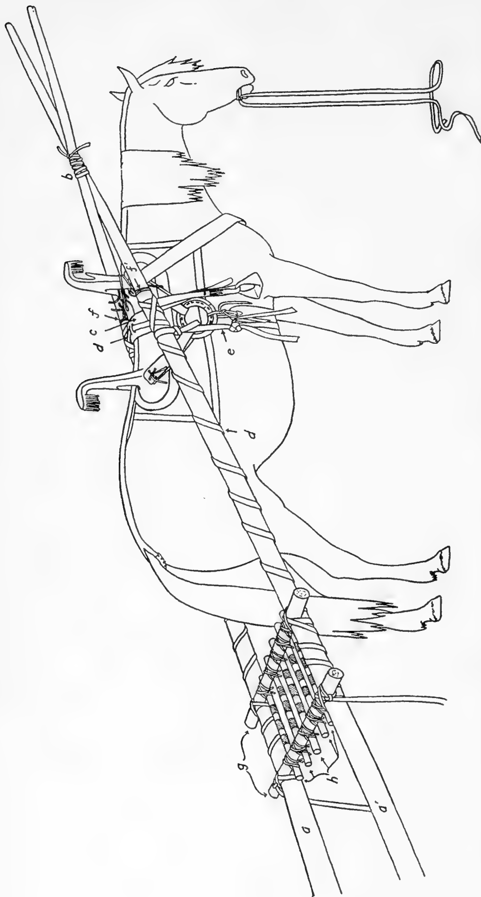
FIGURE 18.—Construction of a Blackfoot horse travois. a, a' , Shafts; b , forward tie; c , rawhide hitch pad; d , rawhide hitch and pole wrapping line; e , girth strap; f, f' , rawhide cord saddle ties; g , primary struts, loading platform; h , secondary struts, loading platform.
