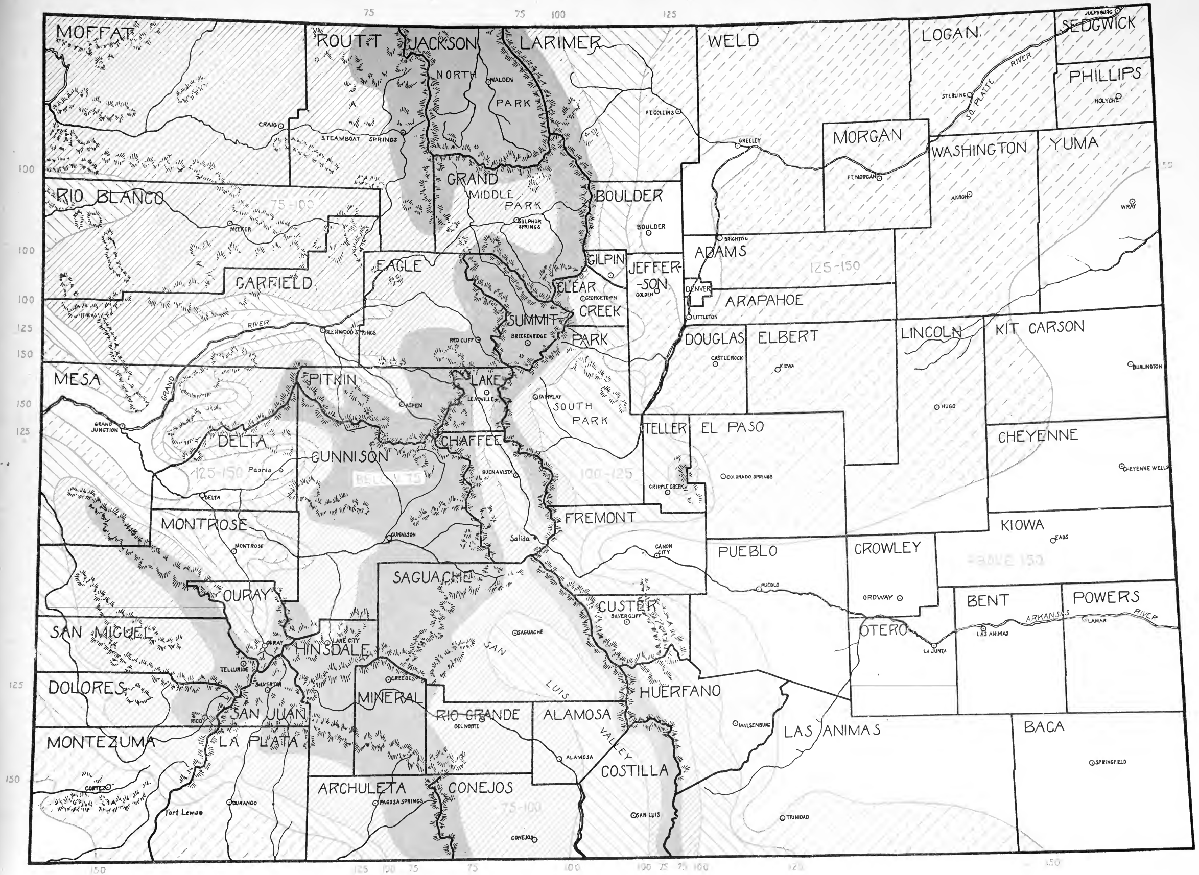
FIG. 5. AVERAGE LENGTH OF FROSTLESS SEASON
