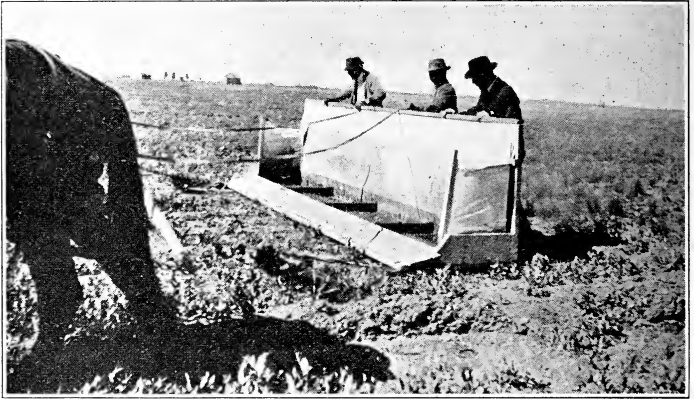
A hopper dozer in action. One of the many machines that was used in the grasshopper campaign, 1916, San Luis Valley. Note the hoppers in the pan. (Original).
