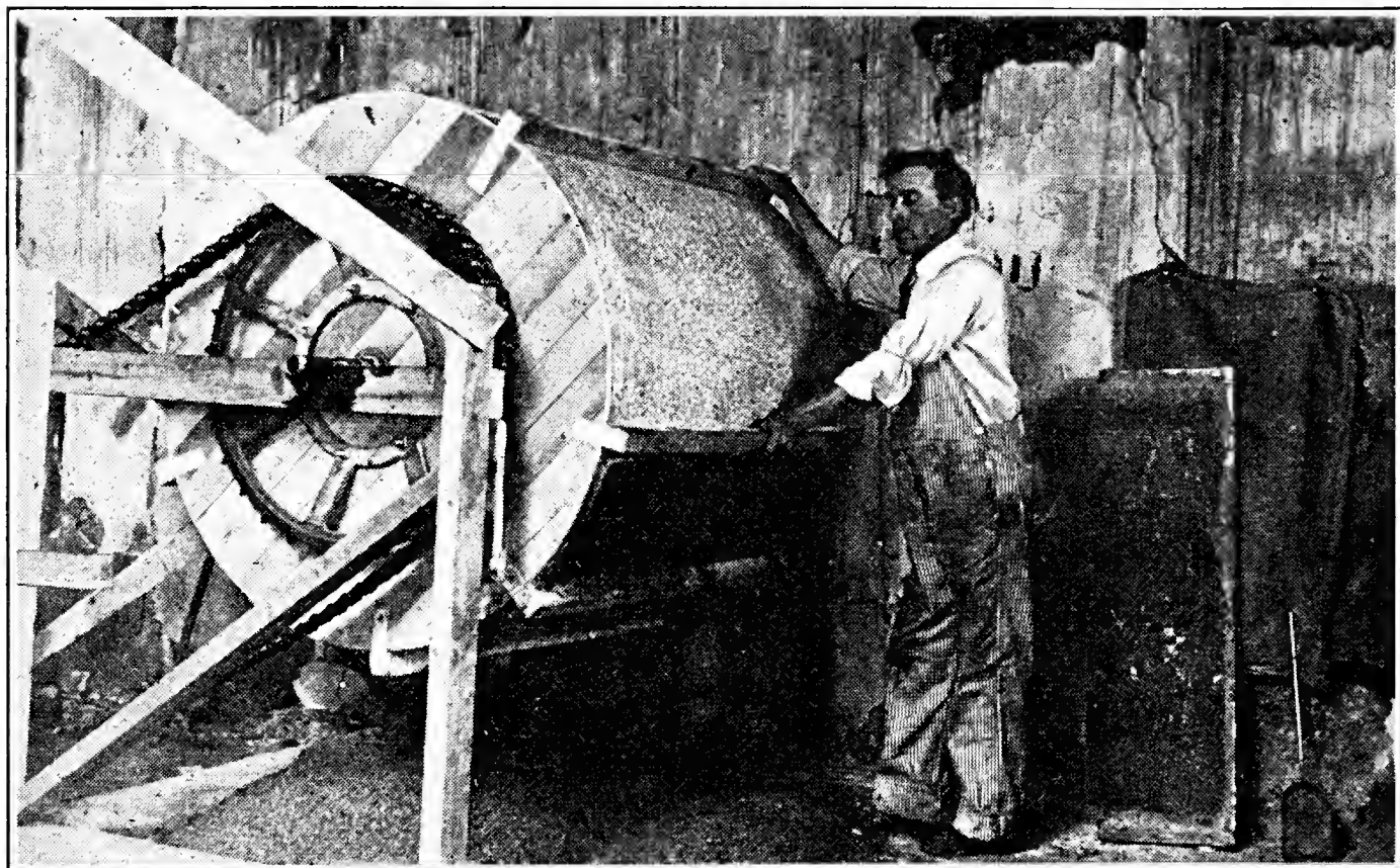
Fig. 8.— Sumpter mixing machine used to mix Paris green-bran mash, Center, Colorado, 1916. Time required to prepare, mix and sack 100 lbs., dry weight, of the bran mash, eight minutes. (Original).
