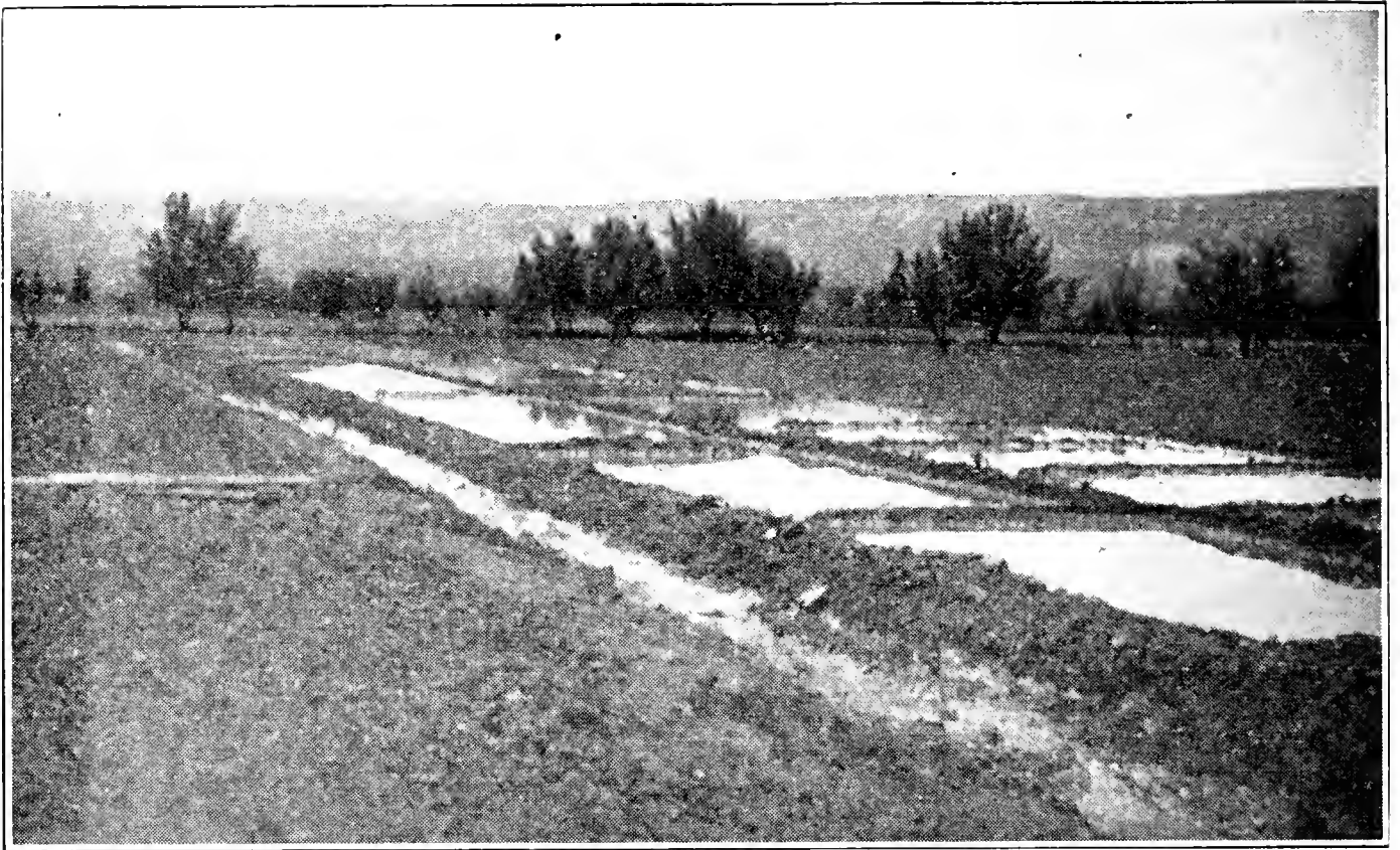
Fig. 1. Method of reclaiming nitre land by flooding
