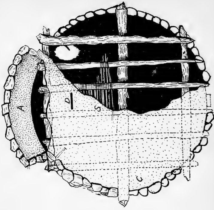
β. SCAFFOLD HOUSE A, large banquette; C, adobe roof covering; D, deflector; S, stick construction supporting roof.
